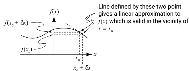
Figure 7: Schematic illustration of the concept of finite differencing
