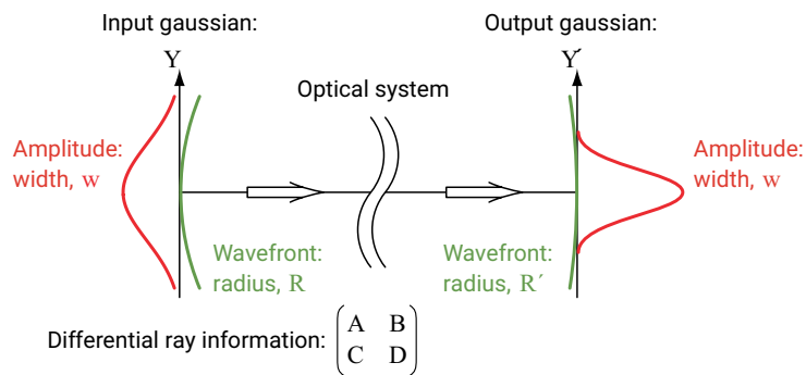
Figure 5: A Gaussian beam propagating through a rotationally symmetric system
