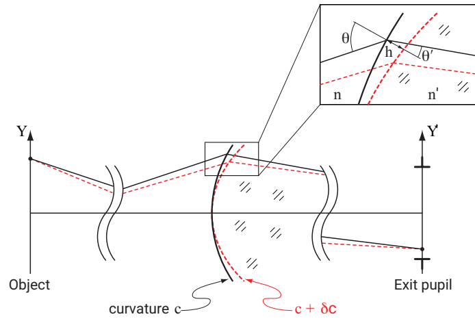
Figure 6: Schematic illustration of a system with a perturbation. A ray through the perturbed system and one through the unperturbed system are shown. These rays both start from the same object point and pass through the same point in the exit pupil
