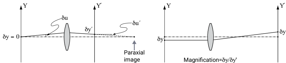
Figure 4: Schematic illustration of the use of differential ray information to determine the paraxial image location and the magnification in an optical system
